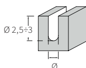
Fresa per cave Slot end mills
